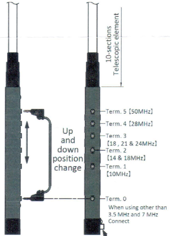
The figure above shows that terminals 0 and 5 are shorted when using 50 MHz.
